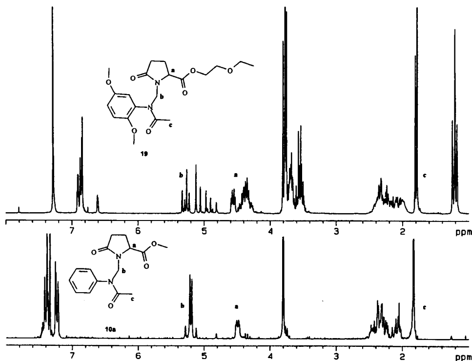
Figure 1. Top: 200 MHz ^1\text{H} spectrum of ester 19 ; bottom 200 MHz ^1\text{H} nmr spectrum of ester 10a .
